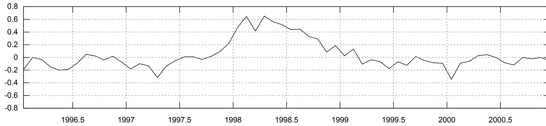
global mean
