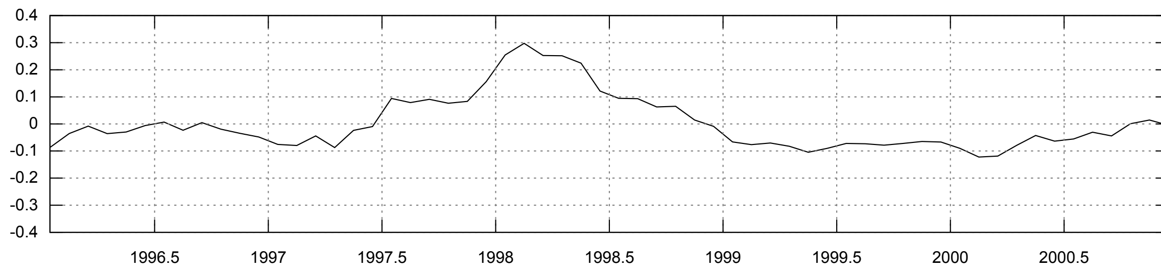
tropical mean
